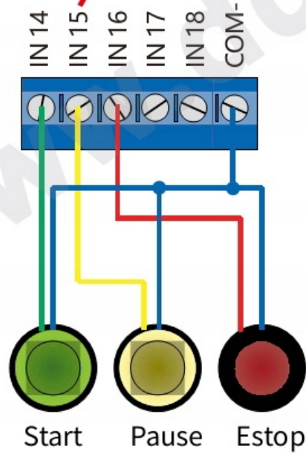
Figure 2-16 The example of external key wiring
