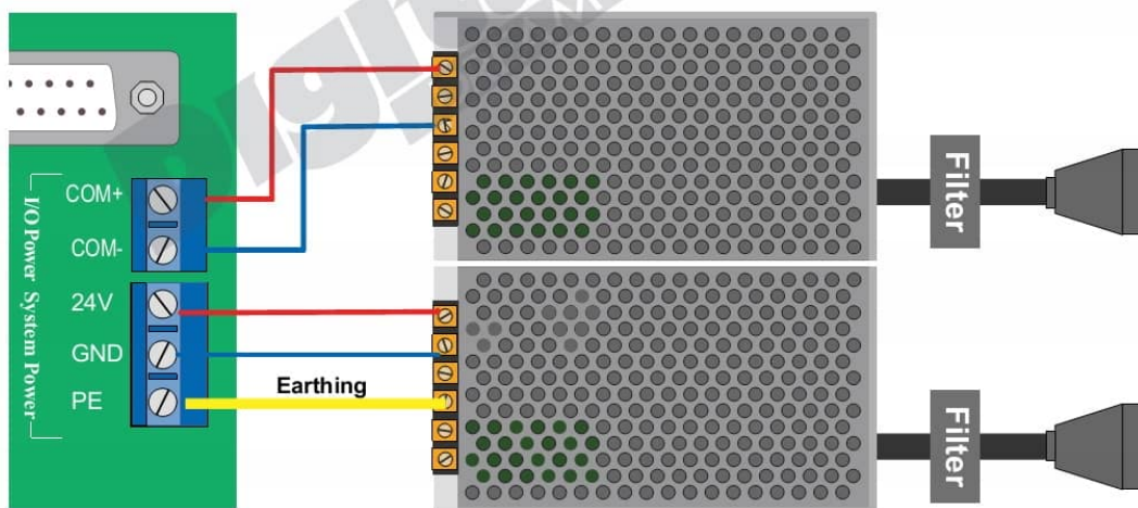
Figure 2-6 DDCS V4.1 Power Supply Wiring Methods
