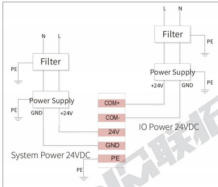
Figure 2-5 DDCS V4.1 Power Supply Wiring Methods
