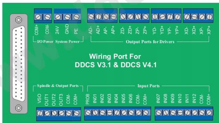
Figure 2-1 DDCCS V4.1 communicate with Wiring board by DB37
