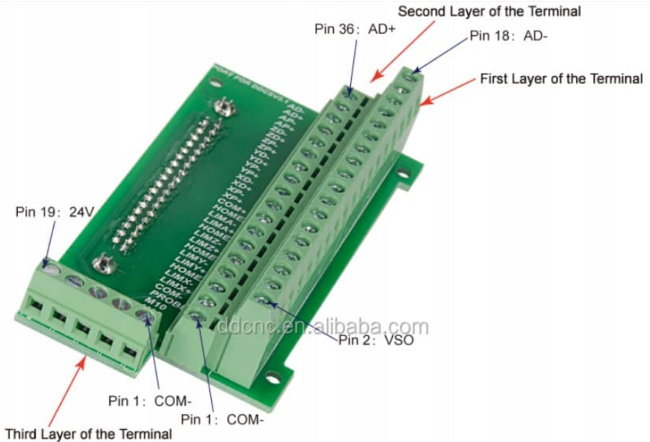
Figure 2-9 3-Layers wiring terminal
