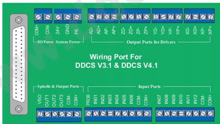
Figure 2-1 DDCC V4.1 communicate with Wiring board by DB37
